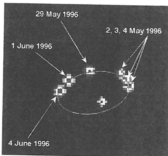
So close, so far. The sharpest optical images ever made, from the Navy Prototype Optical Interferometer, distinguish the two stars in the binary system Mizar A. Separated by just a quarter of the Earth-sun distance, they lie 80 light-years off.
